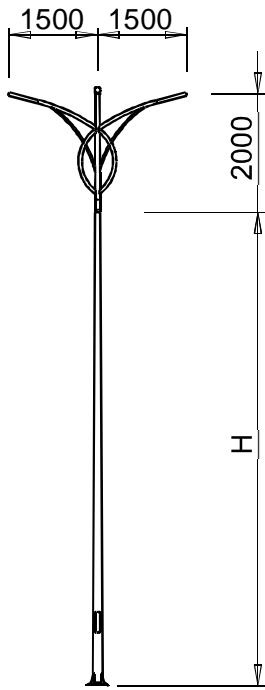
BG...-D78/CKB-01
