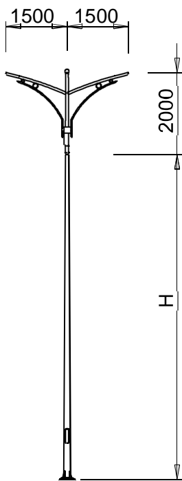
BG...-D78/CKB-04
