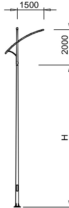
BG...-D78/CDB-05
