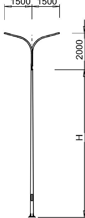
BG...-D78/CKB-06
