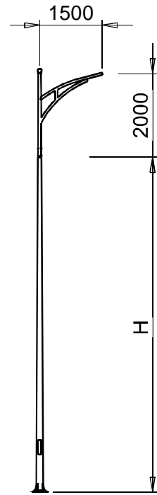
BG...-D78/CDB-03
