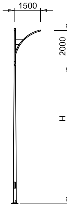
BG...-D78/CDB-02
