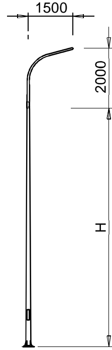
BG...-D78/CDB-06
