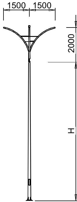
BG...-D78/CKB-02
