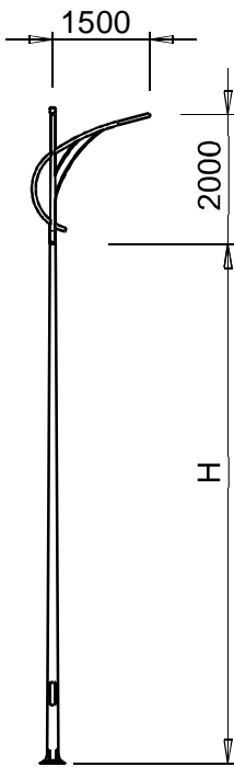
BG...-D78/CDB-01
