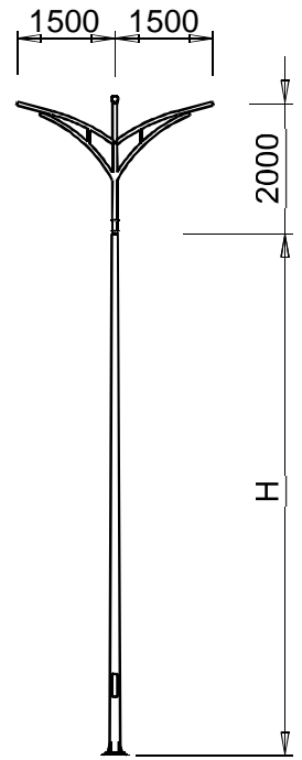
BG...-D78/CKB-03
