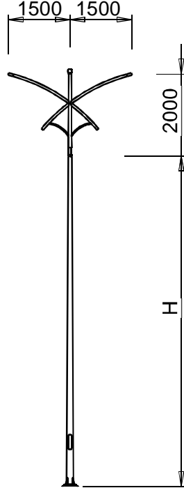
BG...-D78/CKB-05
